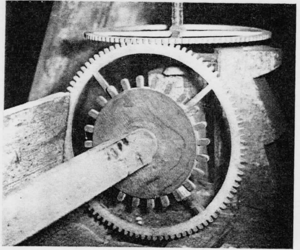
Fig. 14. The wooden shaft of the transmission and also the inoperative wooden wheel to which is secured the multi-toothed metal wheel. Note the primitive construction, the deepening and the crude wooden supporting frame.
