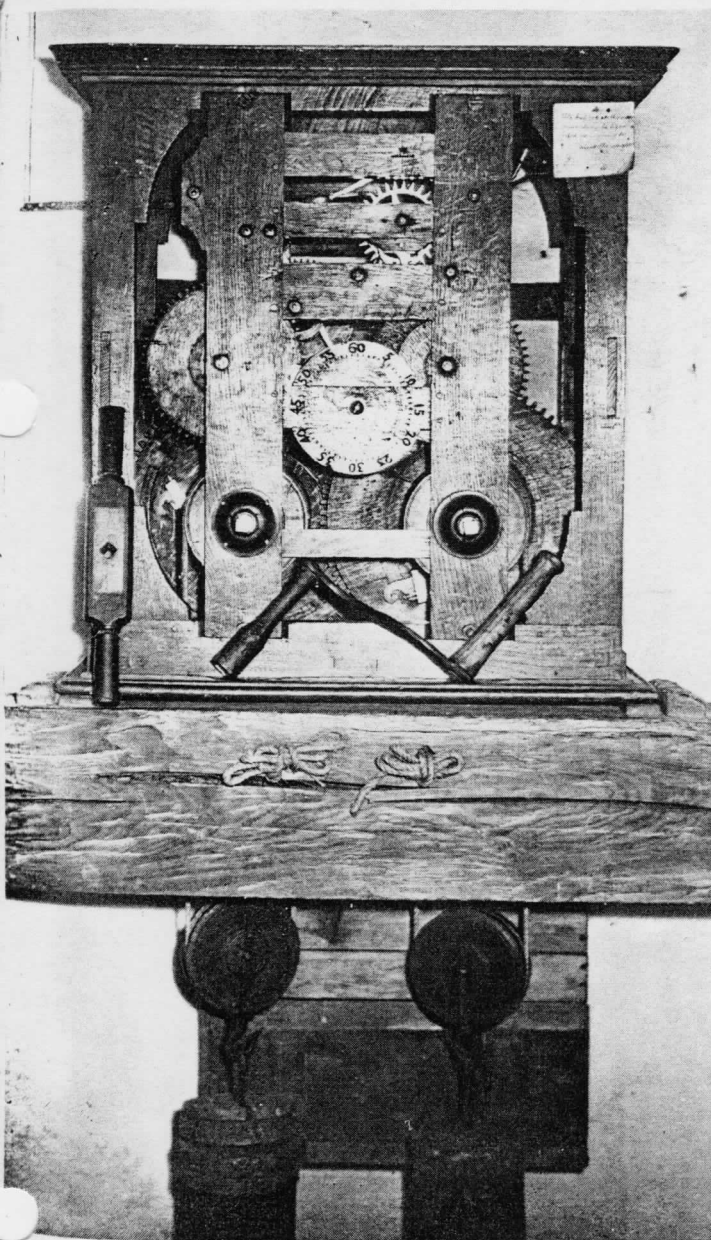
Fig. 3. The mechanism. The escape wheel and one pallet are clearly visible in the upper portion. The original winding handle is on the left.
